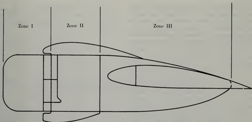
FIGURE 9-7. Fire zone areas.
